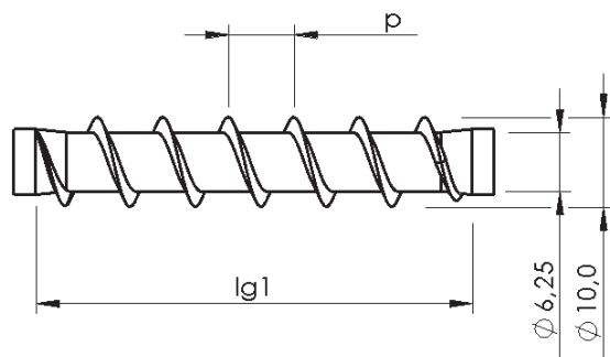
Secondary thread
