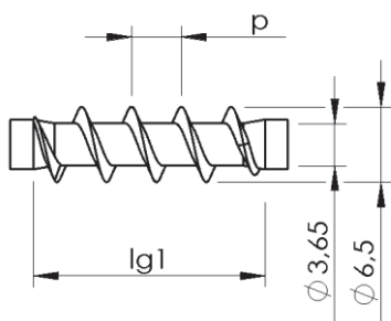
Secondary thread
