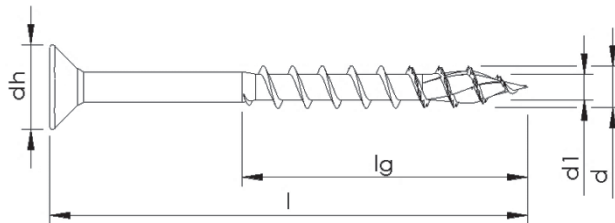
Partial thread without variation, without shank ribs, with toothed tip and milling ribs
