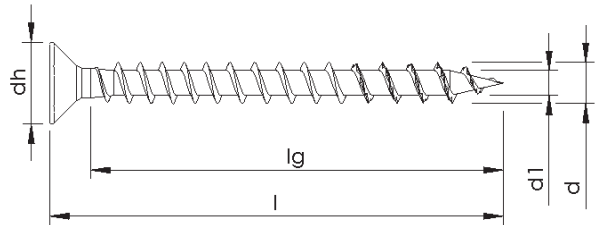
Full thread with variation, toothed tip
